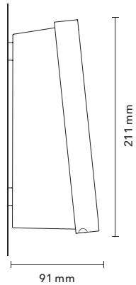
Wall mount (WM-Box)
